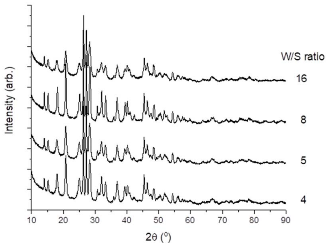
Figure S2. XRD patterns for the samples prepared by microemulsion using different W/S ratios.
