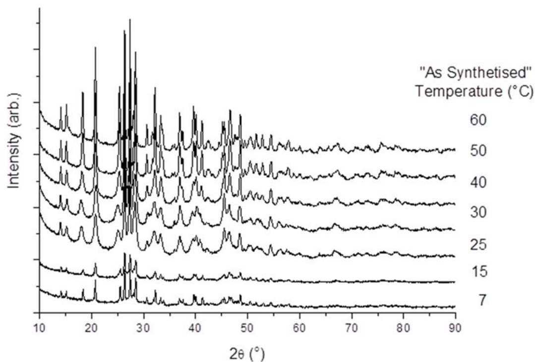
Figure S1. XRD patterns for the samples prepared by microemulsion using different temperatures of synthesis.
