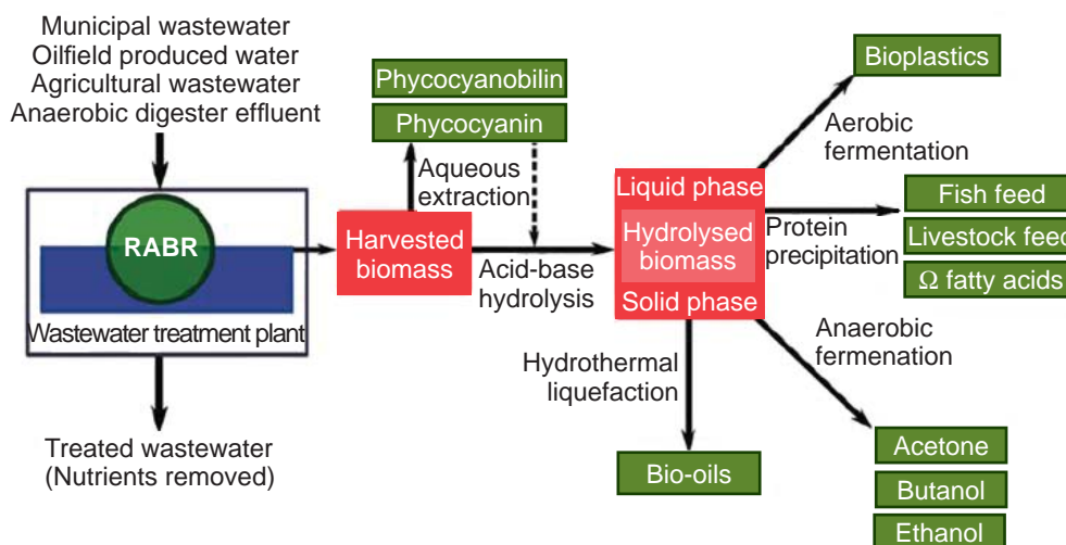
Fig. 1. Coupling wastewater treatment with algae production (Reproduced by permission of Springer India)
